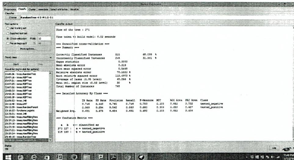
Fig 3: Random tree
