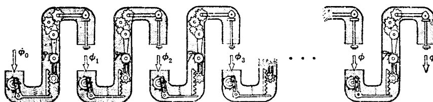
Figure 5. The "S-machine"
