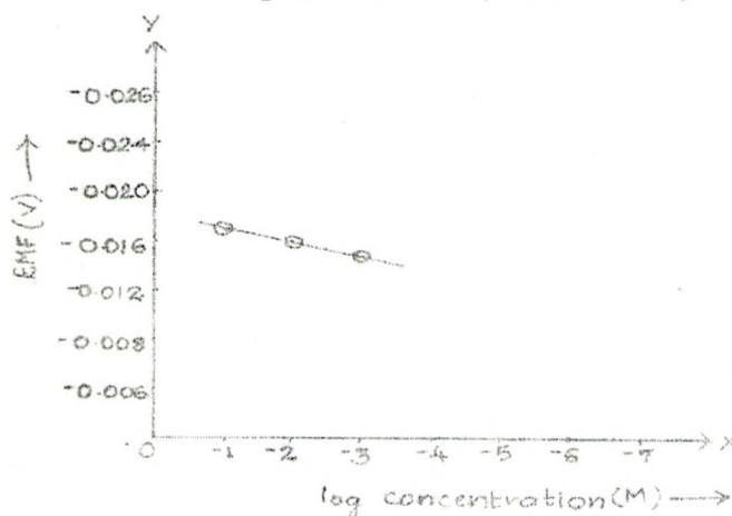
Electrode response sodium (electrode-III)
