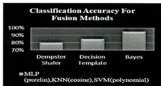
Figure 2: Comparison of classification accuracy with fusion methods
