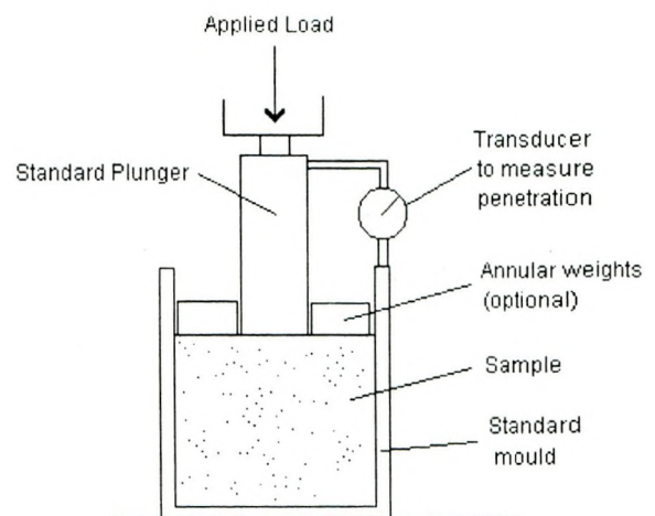
Figure 1: California bearing ratio tester.
