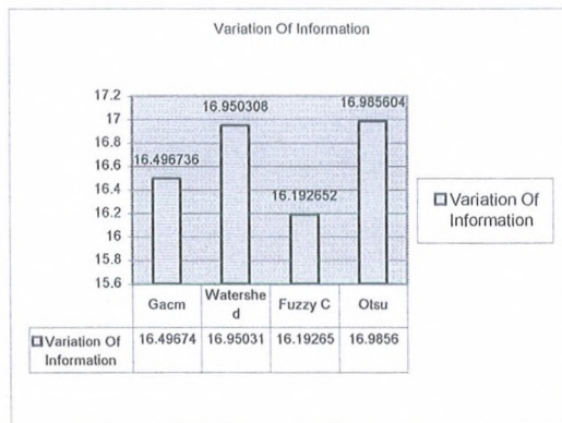
Figure 4: Evaluation graph using Variation Of Information
