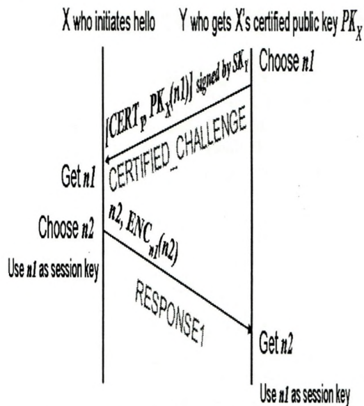
Figure 4: Three Way Challenge-Response Handshake
