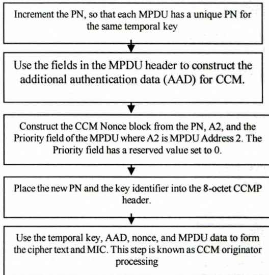
Figure 5: CCMP encapsulation algorithm
