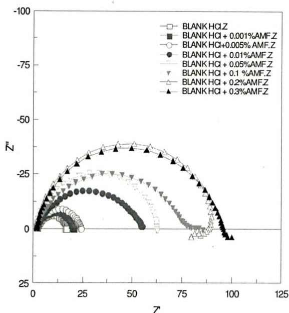
Figure: 6 Nyquist Plot of mild steel in 1M HCl
