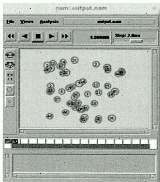
Figure 1. Network Model
