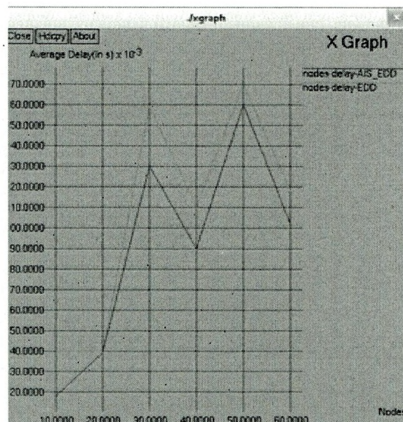
Figure 5. Average Delay
