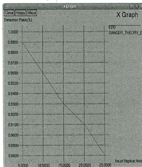
Figure 8. Detection Ratio
