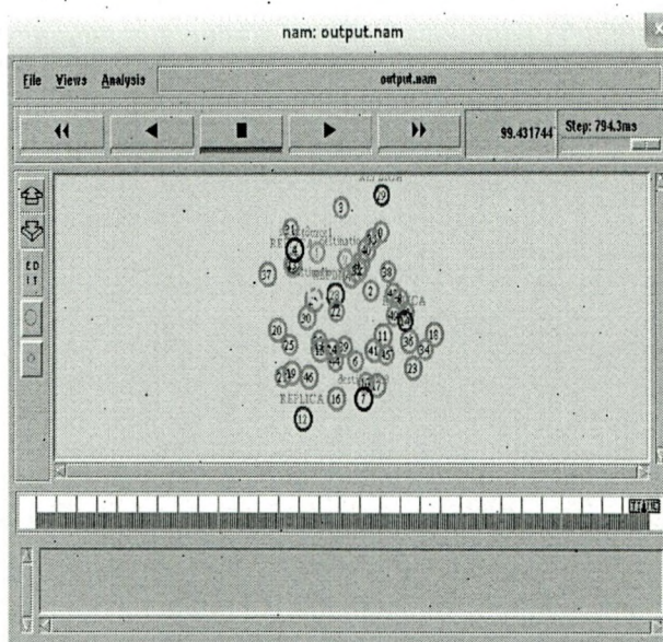
Figure 2. Threat Model
