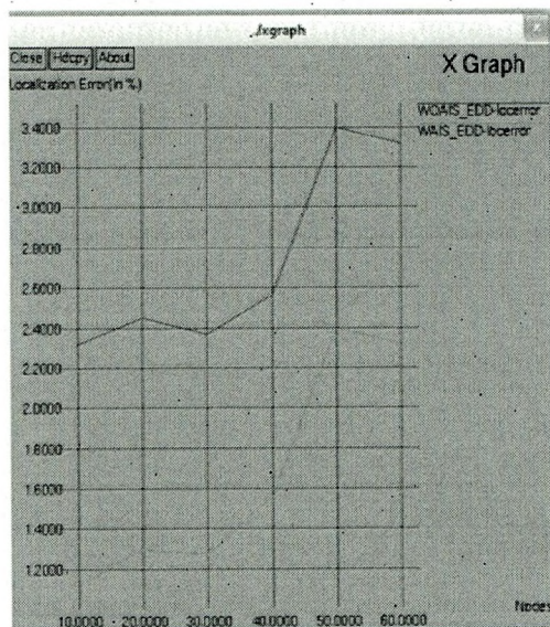
Figure 7. Localization Errors
