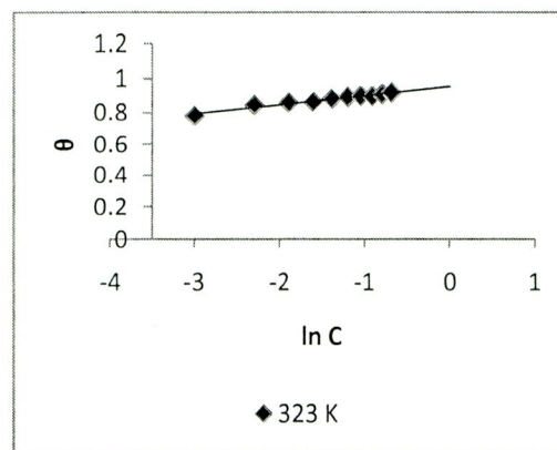
Figure 3: Temkin adsorption isotherm
