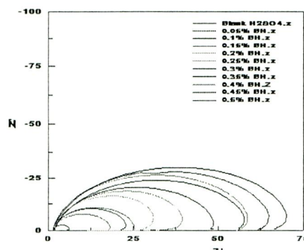
Figure 7: Nyquist plot
