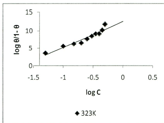
Figure 2: Langmuir adsorption isotherm
