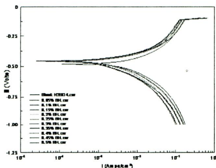
Figure 6: Tafel plot
