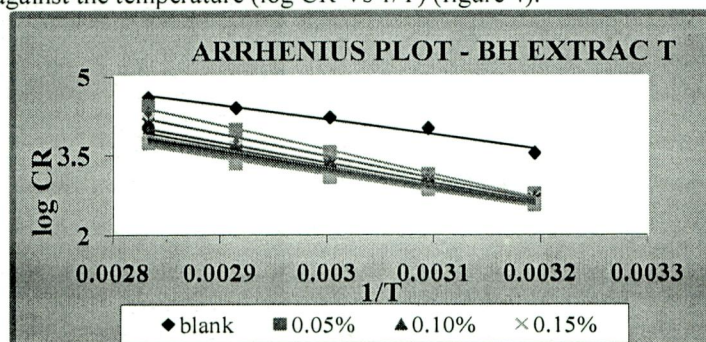
Fig 4 Arrhenius plot
