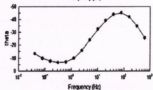
Fig-6-Bode Plot
