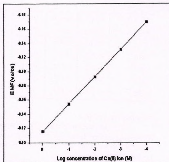
Fig-4-Electrode Response
