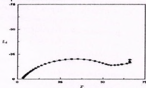
Fig-5-Nyquist plot
