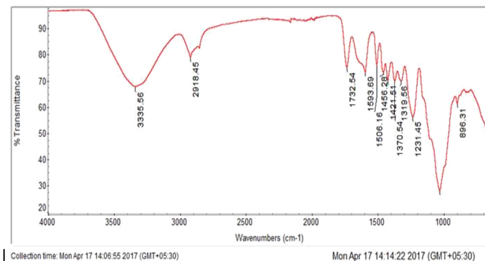
Fig 3: FTIR Analysis
