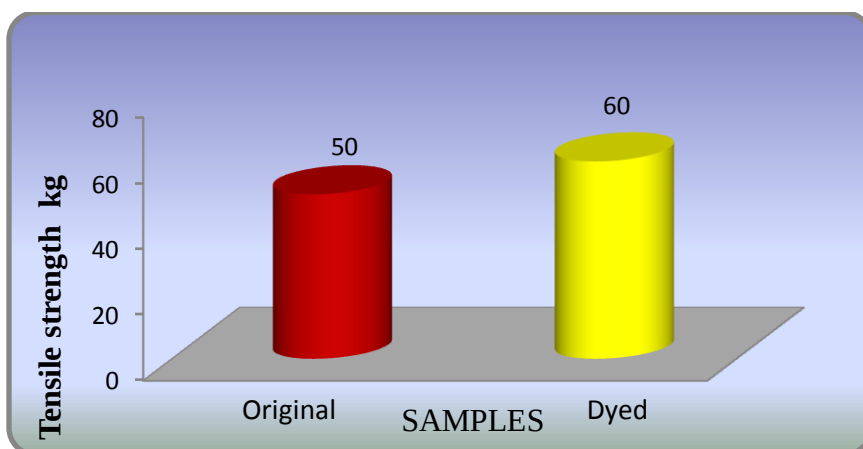
Figure 2 Fabric Strength
