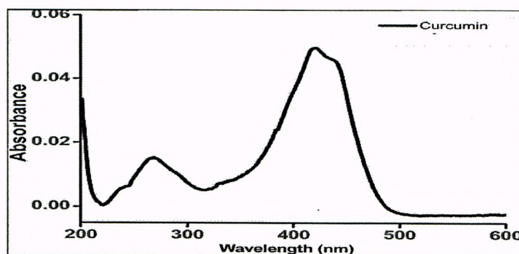
Fig. 1: UV-Visible spectrum of standard curcumin
