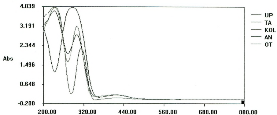
Fig. 2: Comparison of UV-Visible spectra of curcumin extracted from turmeric samples from 5 different states (UP, TA, KOL, AN and OT)
