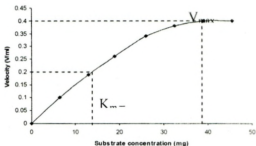
Fig. 5. Michealis - Menten Kinetics
