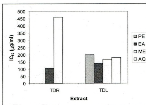
Fig. 1: \text{IC}_{50} values for DPPH free radical scavenging activity of Trianthema decandra roots and leaves
