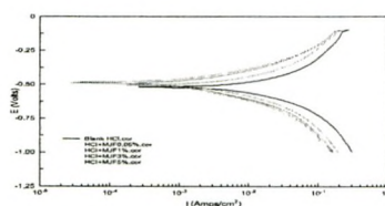
Figure 3: Potentiodynamic polarization curves for mild steel in 1M HCl for various concentrations of MJF extract
