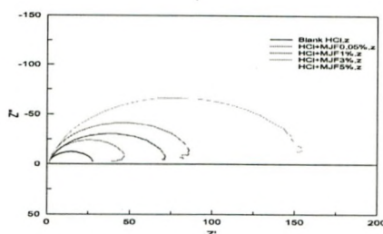
Figure 4: Nyquist plots for mild steel in 1M HCl in the absence and presence of various concentrations of MJF extract
