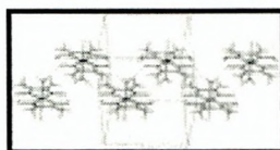
Fig. 2. Part of the crystal structure of the title compound showing the formation of one dimensional chain through O3—H3\cdots O1^{ii} hydrogen bond extending along [010] direction [Symmetry codes: (i) x, -y + 1/2, z ; (ii) -x + 1, y - 1/2, -z + 1 ].
